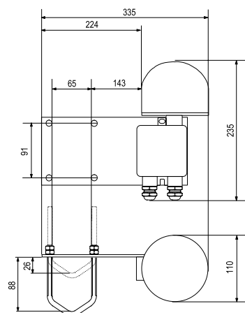
CEL-MS-60 Mounting
