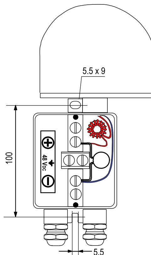
CEL-10-48-F terminal box
